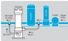
Illustration of Model 300 Feeder
