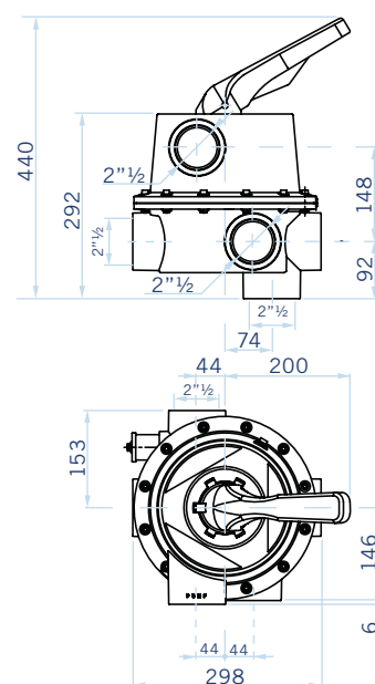
24838. Modelo sin enlace a filtro / Model without connection to filter
